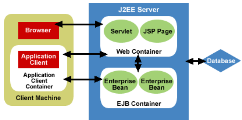
Figure 1: Application Server Overview
