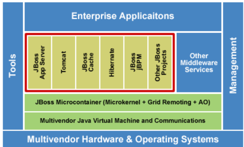
Figure 3 The Architecture of JBoss AS and JEMS
